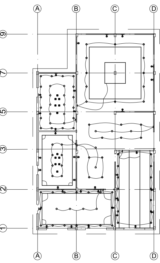
Key Plan: Electrical Partial Plan
