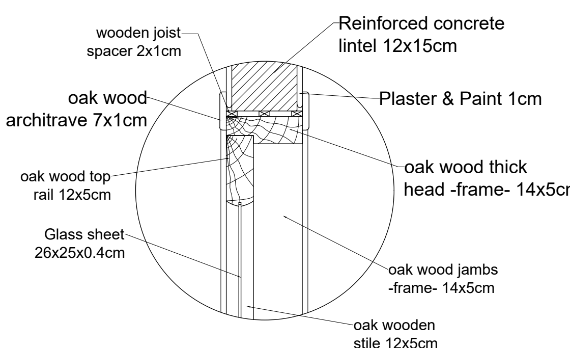
Typical Detail for Wooden Paneled door Detail A-A Scale 1:5
