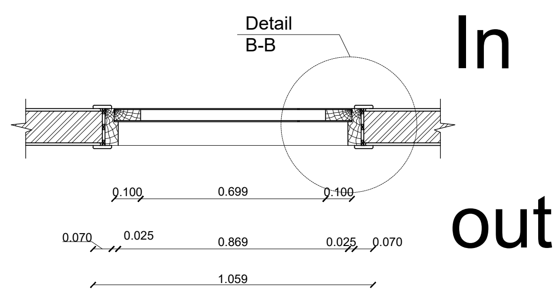
Typical Detail for Wooden Flush door Transferal section B-B'/D3 Scale 1:10
