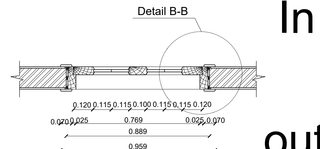
Typical Detail for Wooden Paneled door Transferal section B-B'/D1 Scale 1:10
