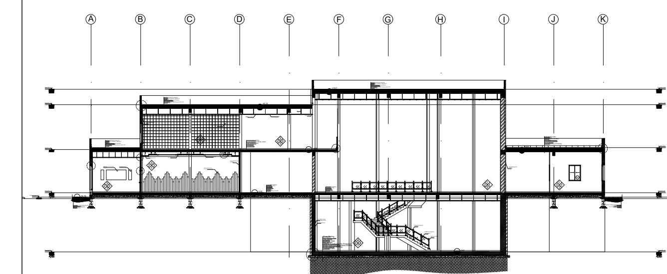
Key Section: Section A-A'
