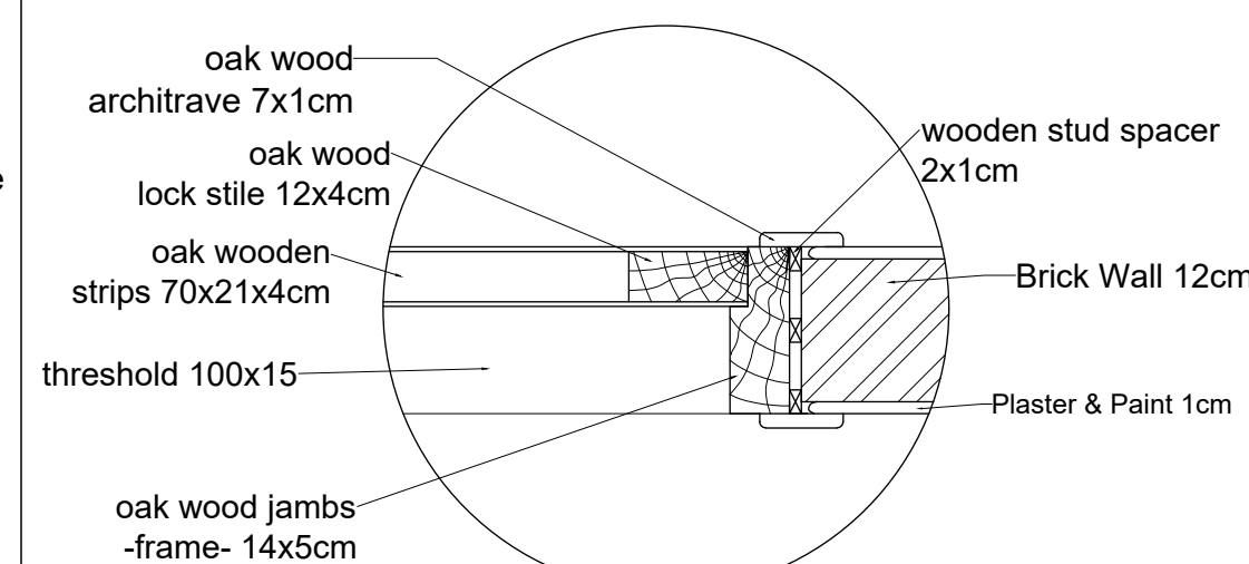
Typical Detail for Wooden Flush door Detail B-B Scale 1:5
