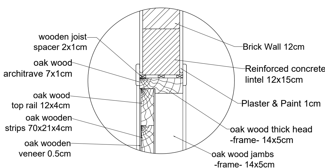
Typical Detail for Wooden Flush door Detail A-A Scale 1:5
