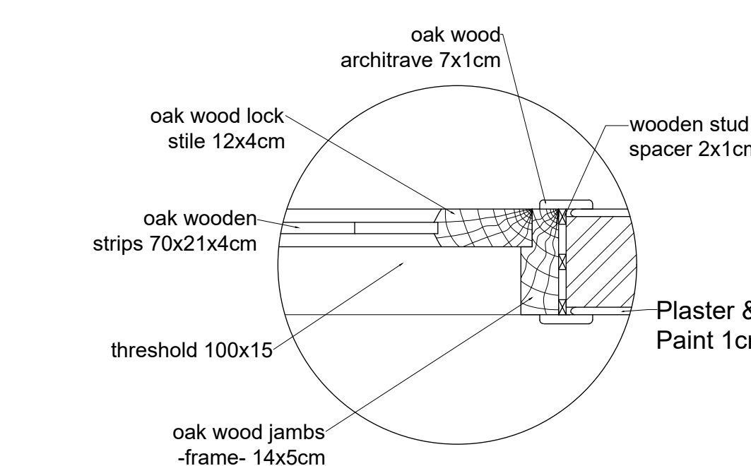
Typical Detail for Wooden Paneled door Detail B-B Scale 1:5
