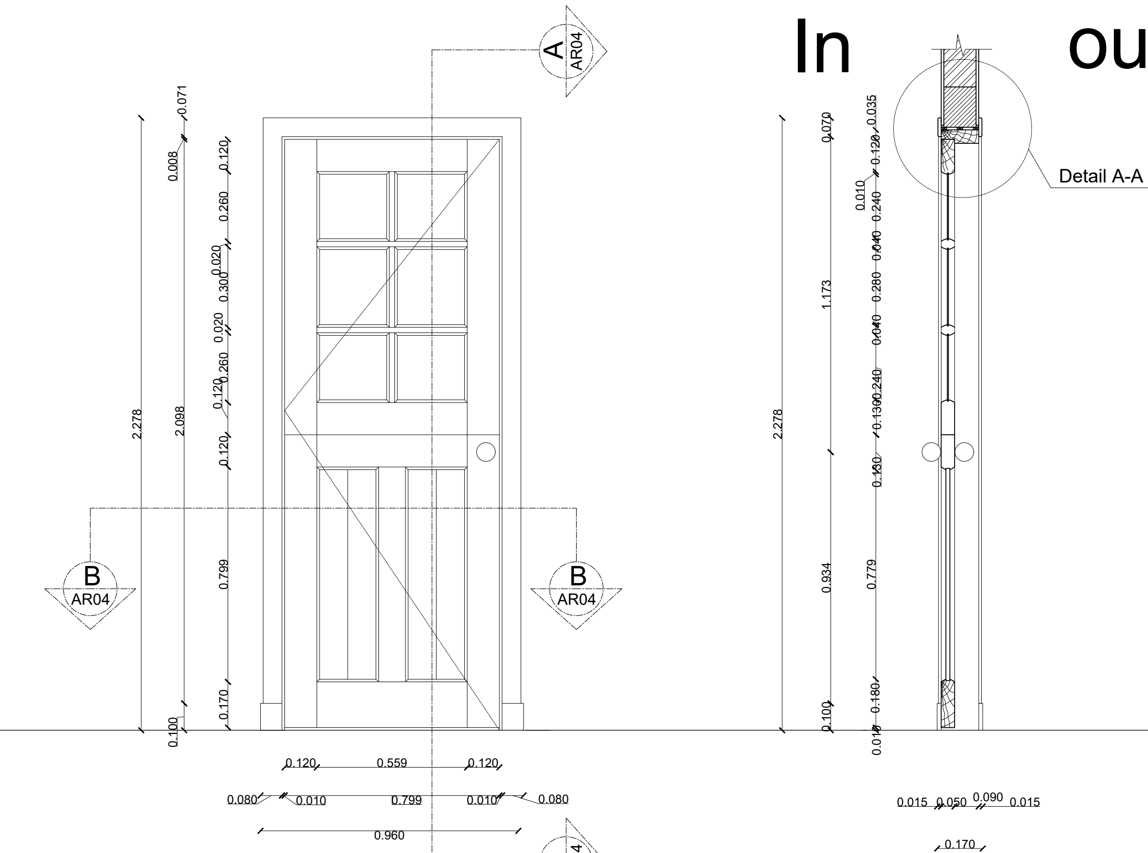
Typical Detail for Wooden Paneled door longitudinal section A-A'/D1 Scale 1:10
