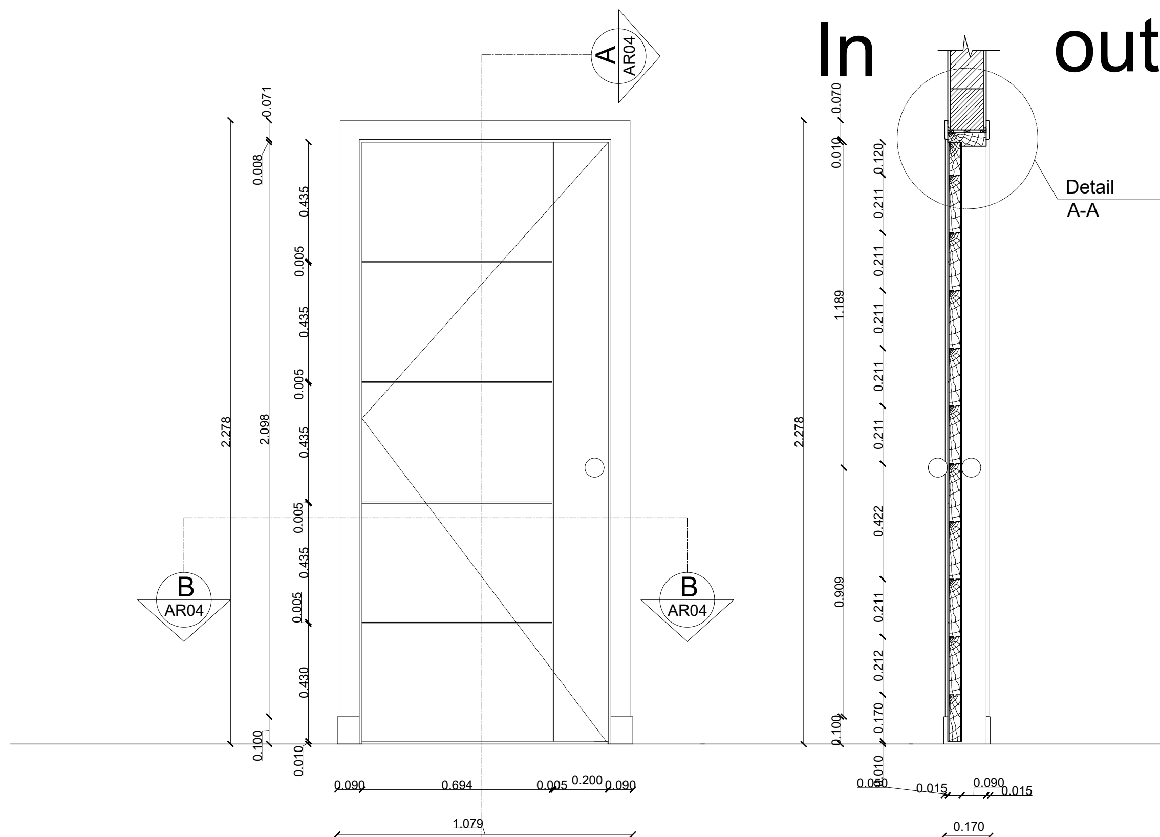
Typical Detail for Wooden Flush door Door Elevation/D3 Scale 1:10
